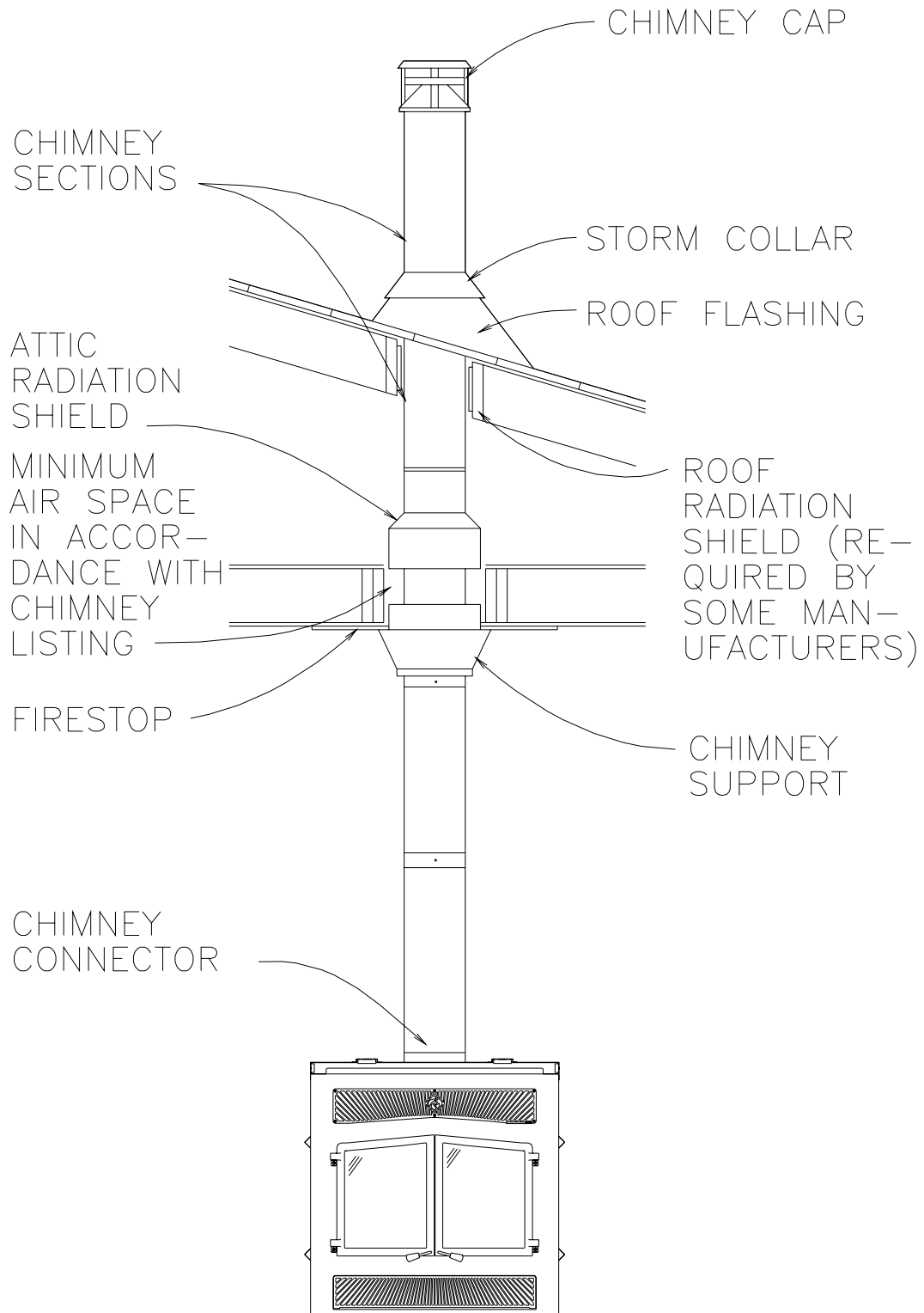
FIGURE 25: AC CHIMNEY
