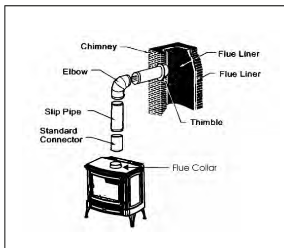
A. Chimney connection is a freestanding installation
