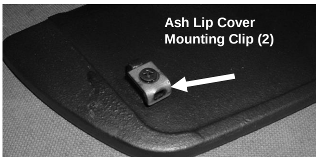
Photo 21 – Ash Lip Cover Mounting Clip Detail
