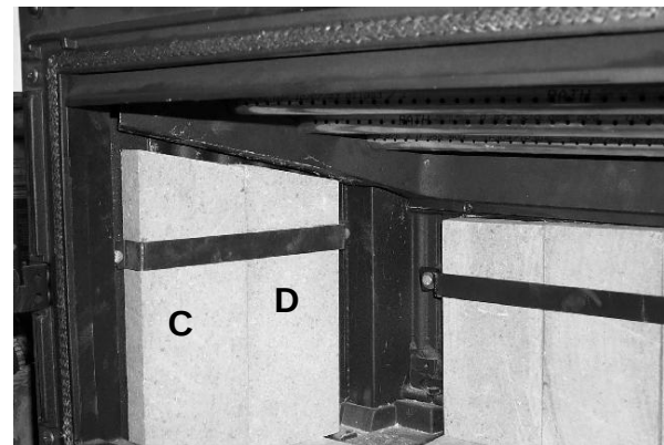
Photo 15 – Left and Right Side Stones
