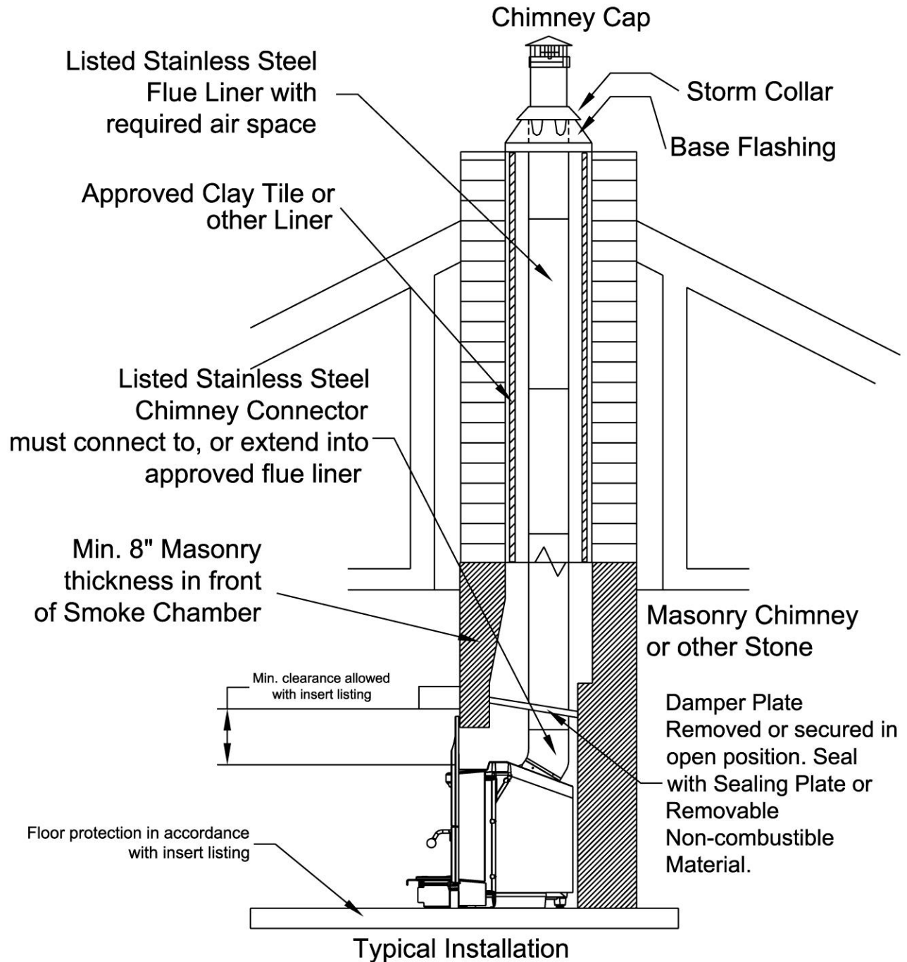
Figure 5 – Connecting to a masonry chimney
