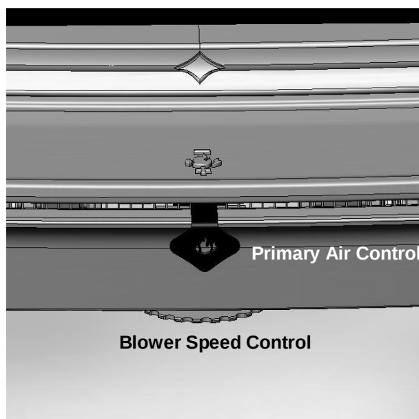
Figure 8 – Primary Air, & Blower Speed Controls
