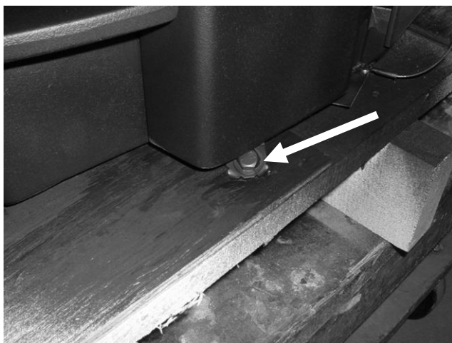
Photo 1 – Pallet Mounting Clip Detail (Right Front Shown - Façade Installed)
