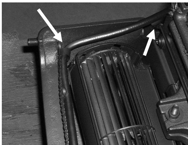
Photo 29 – Correctly Routed Cord Detail
