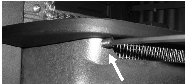
Photo 25 – Set Screw Detail
