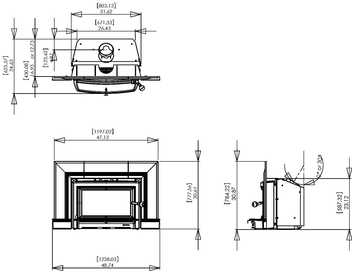
Figure 1 – Clydesdale Dimensions
