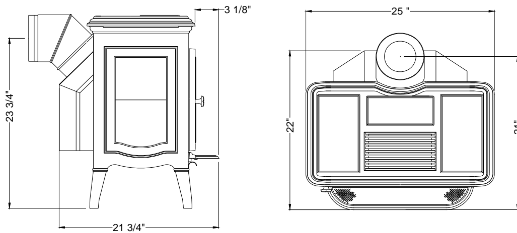
Figure 2 - Santa Fe Dimensions
