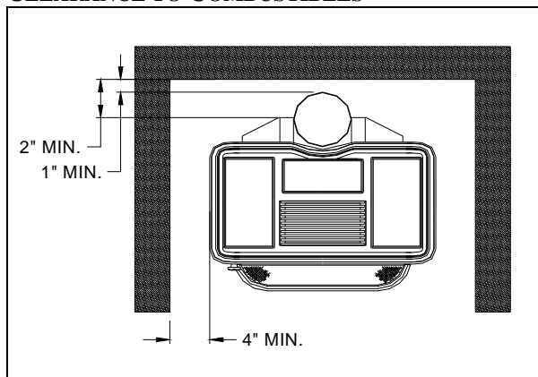
Figure 3 - Rear and side wall clearances
