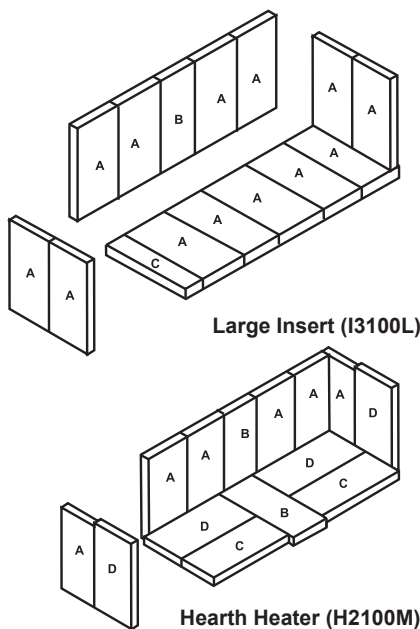
Hearth Heater (H2100M)
