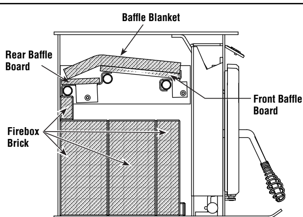
Figure 4 - Side Cut-A-Way View of Firebox
