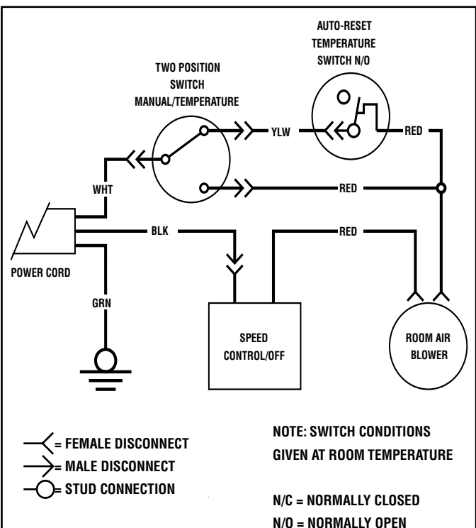
Figure 12 - Blower Wiring Schematic
